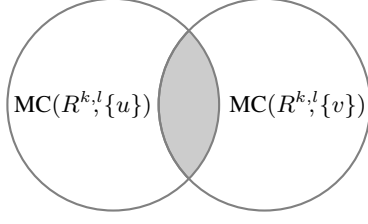
Figure 1. An illustration of MC(R^{k,l}, u \cap v) .
